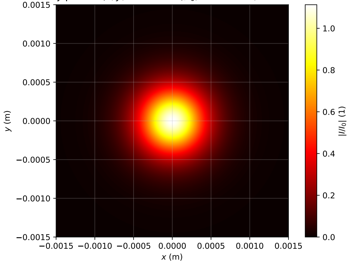
Intensity profile I(x, y, z = 2.946m)/I_0 , P_{in}=0.8P_{cr} , artificial time
